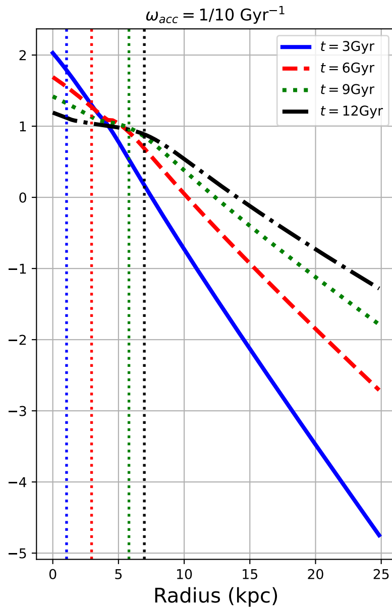
\Sigma_{gas} vs r for different t and t_{acc}
